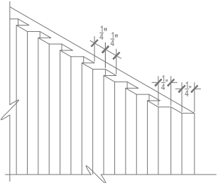
Detail / Dimensions
