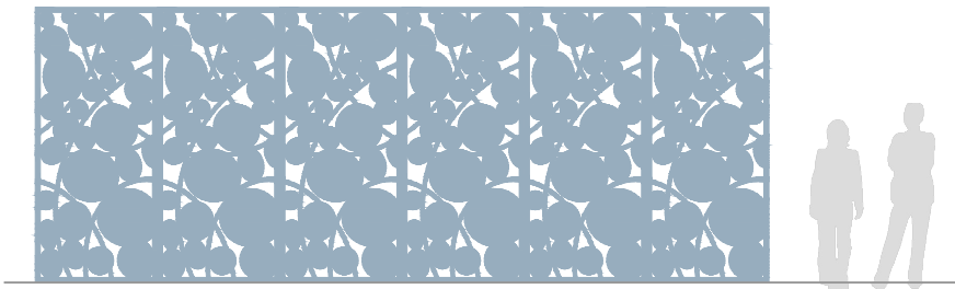
Pattern Iteration
