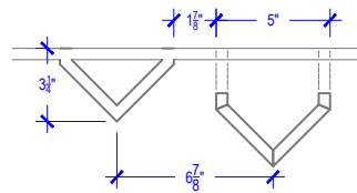
Ridge Dimensions
